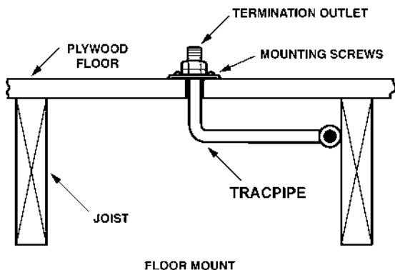
Figure: 4-26 Support Device Flange Termination Outlet
